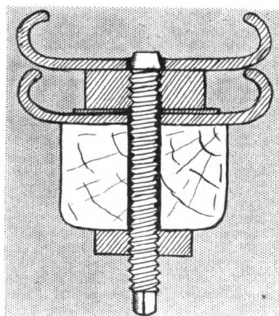
Cross Section Hard Spare Wheel.
